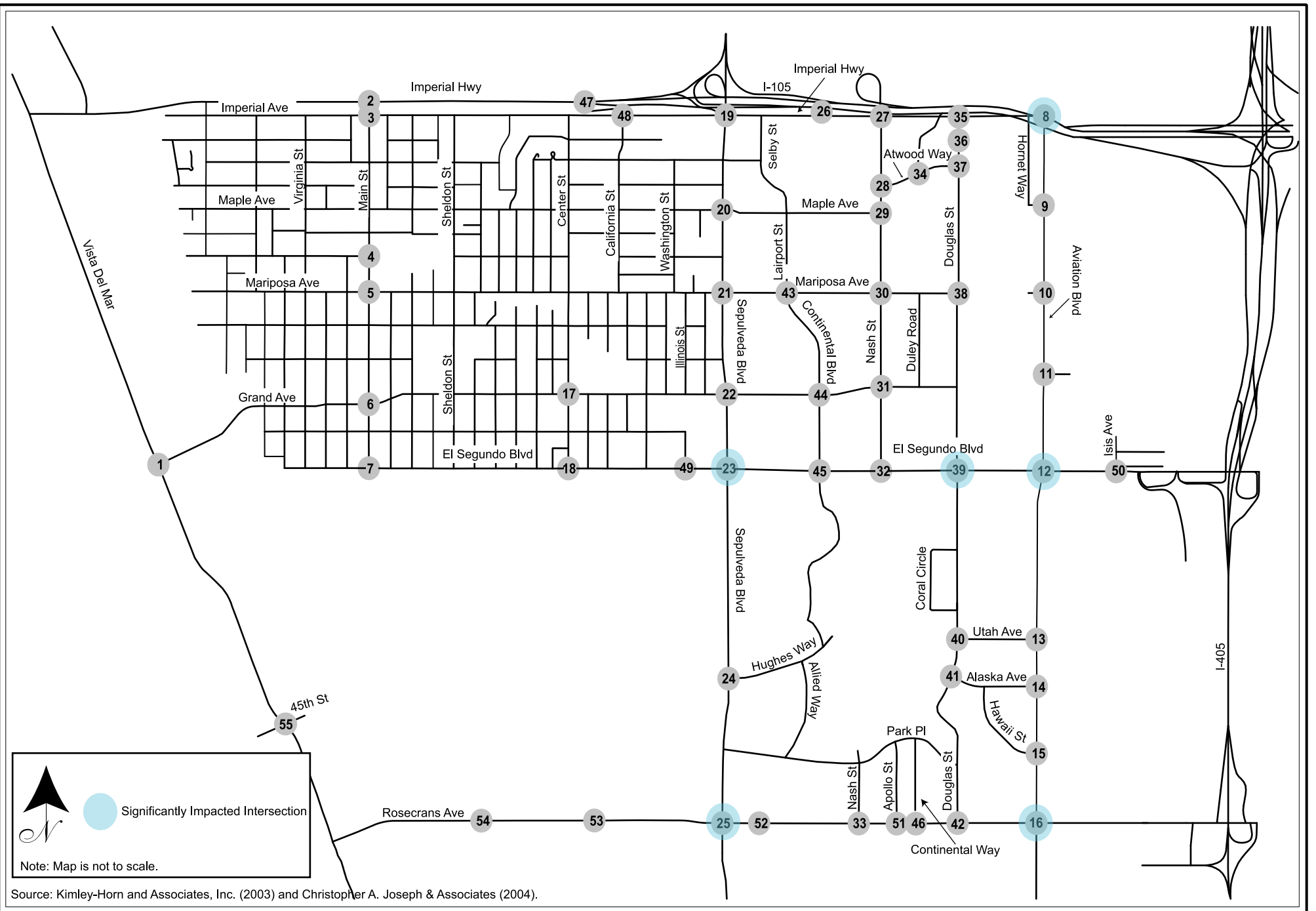
Figure IV.B-3 Year 2025 Significantly Impacted Intersections
